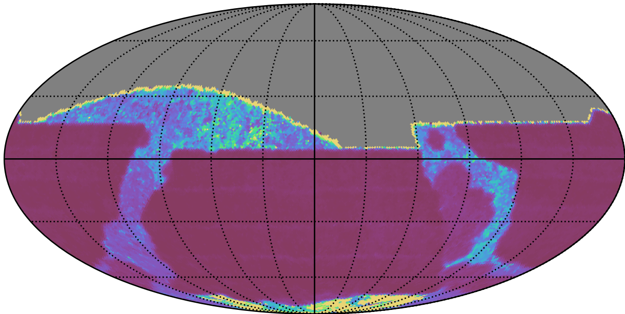
ddf_loaded_half_fl15_v3.4_10yrs All sky z band: Median Inter-Night Gap
