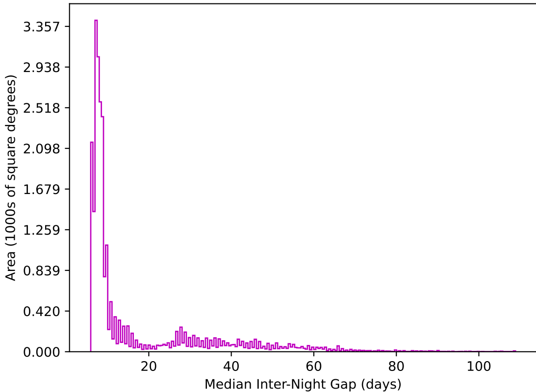
ddf_loaded_half_fl15_v3.4_10yrs All sky z band: Median Inter-Night Gap
