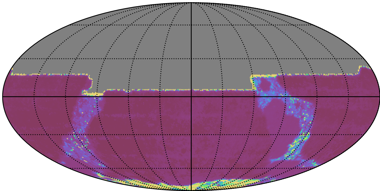
ddf_loaded_half_f15_v3.4_10yrs All sky y band: Median Inter-Night Gap
