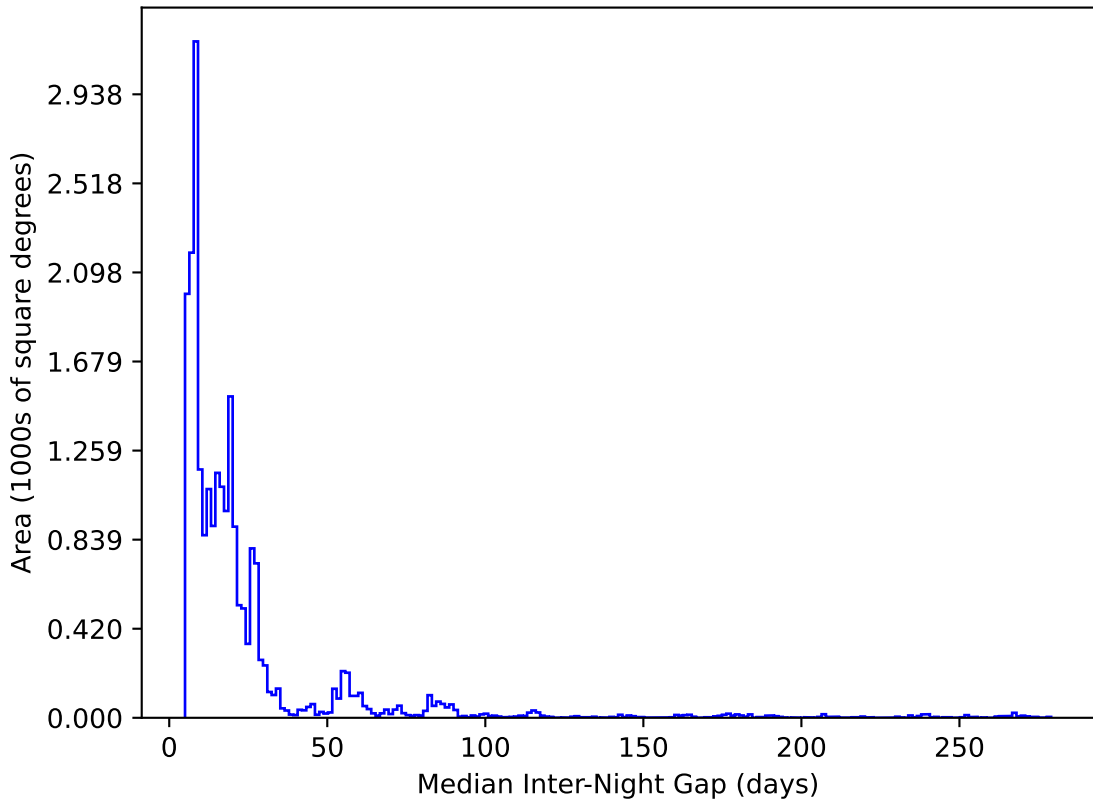
ddf_loaded_half_fl15_v3.4_10yrs All sky y band: Median Inter-Night Gap
