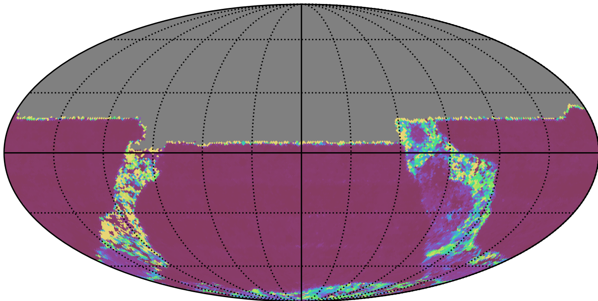
ddf_loaded_half_fl15_v3.4_10yrs All sky u band: Median Inter-Night Gap
