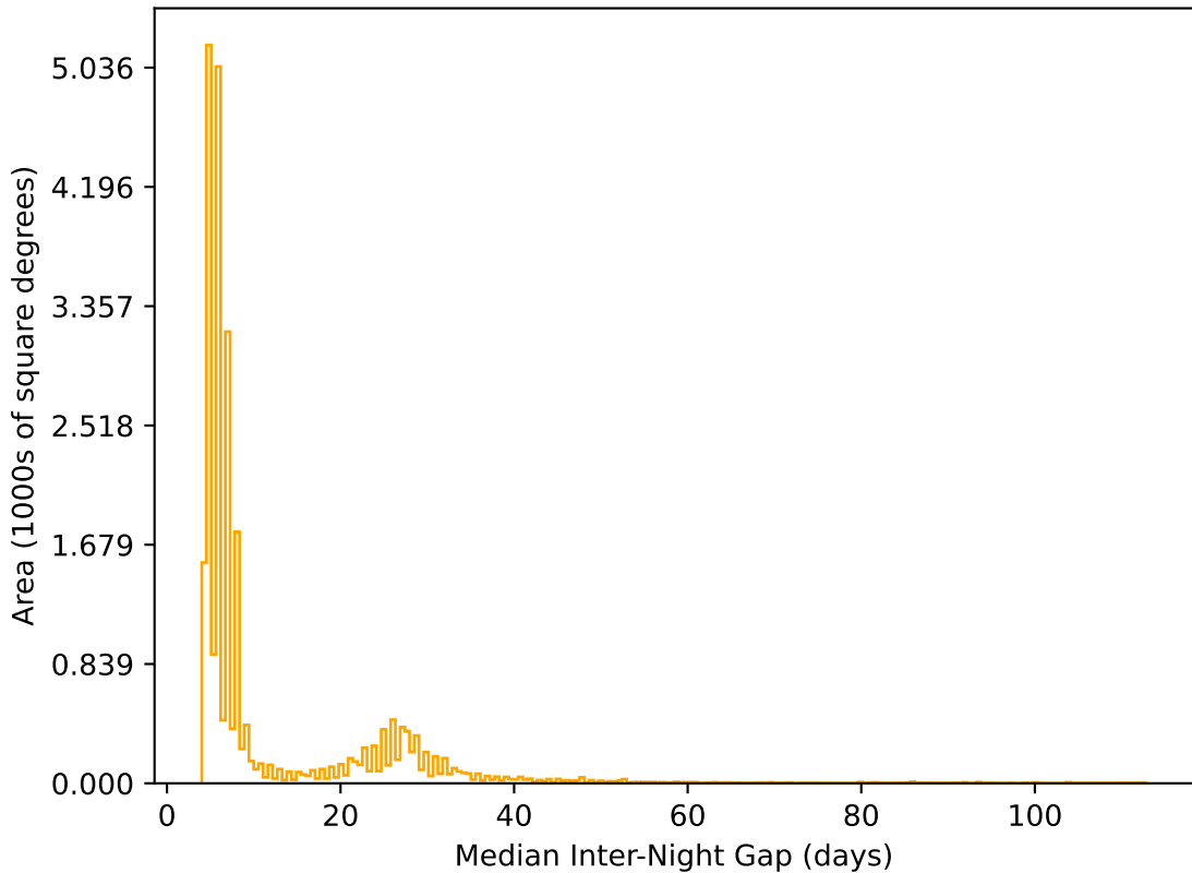
ddf_loaded_half_fl15_v3.4_10yrs All sky r band: Median Inter-Night Gap
