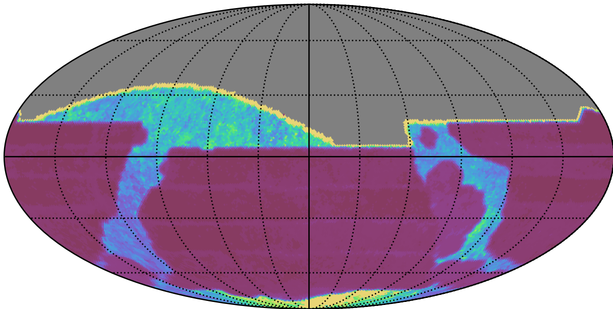
ddf_loaded_half_fl15_v3.4_10yrs All sky all bands: Median Inter-Night Gap
