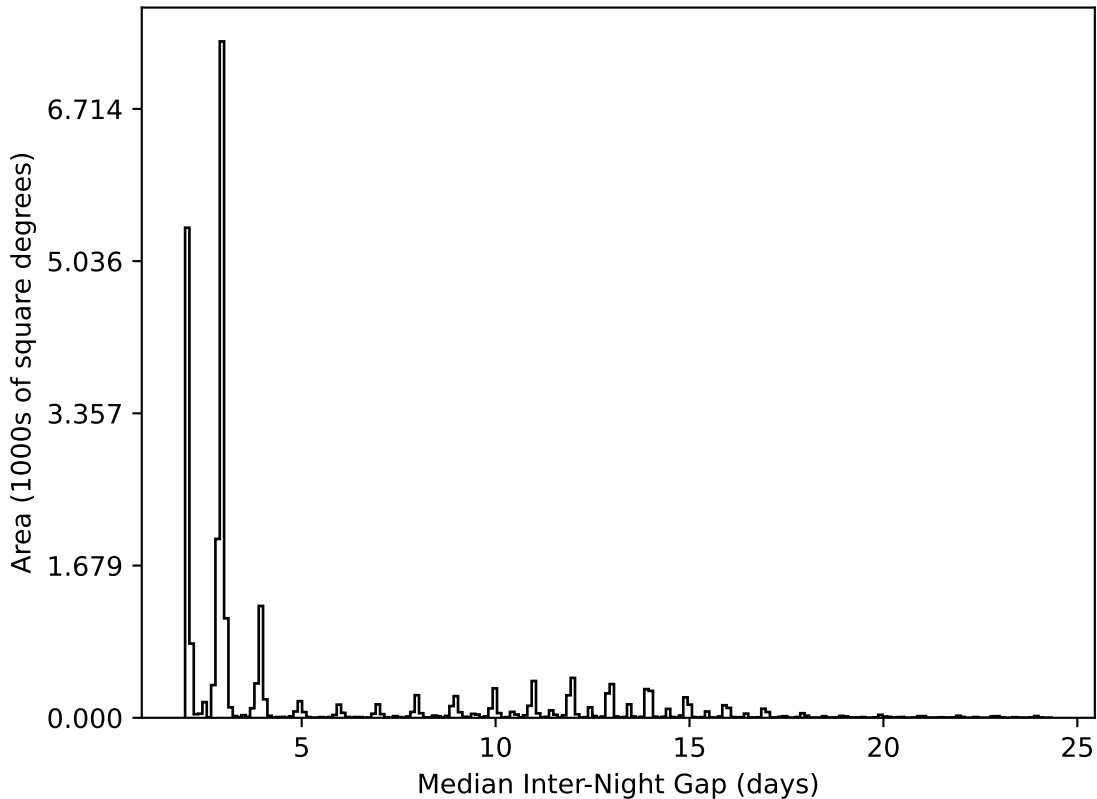
ddf_loaded_half_fl15_v3.4_10yrs All sky all bands: Median Inter-Night Gap
