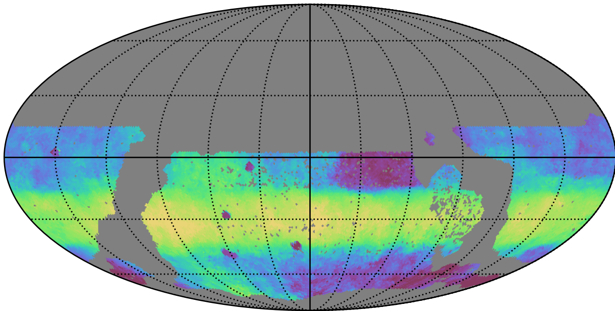
ddf_loaded_half_fl15_v3.4_10yrs WFD z band: Median HA
