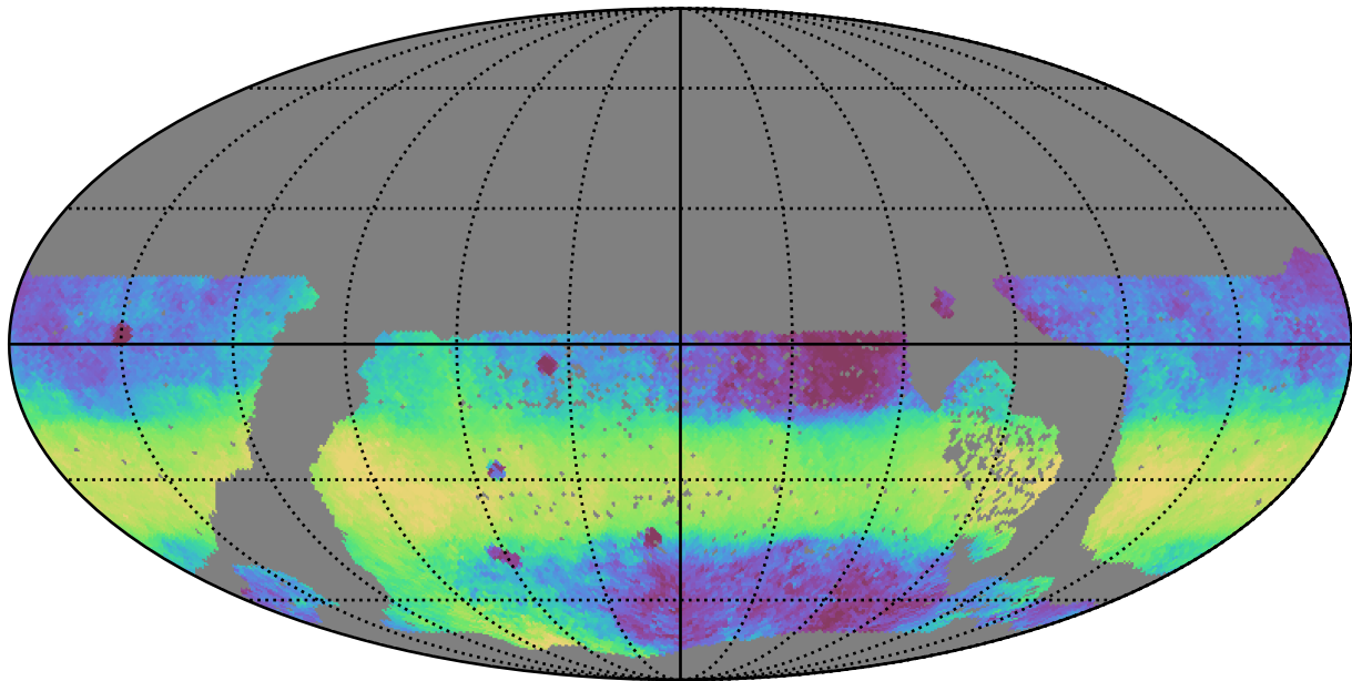
ddf_loaded_half_fl15_v3.4_10yrs WFD y band: Median HA
