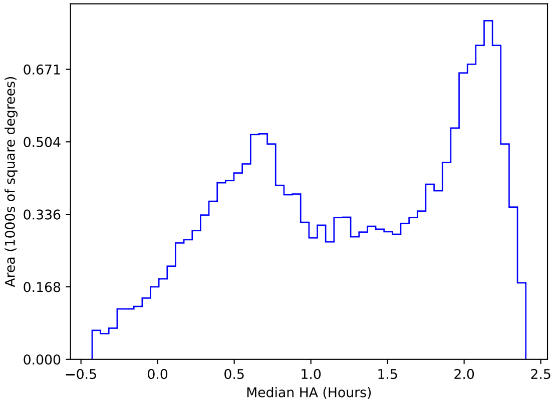
ddf_loaded_half_fl15_v3.4_10yrs WFD y band: Median HA
