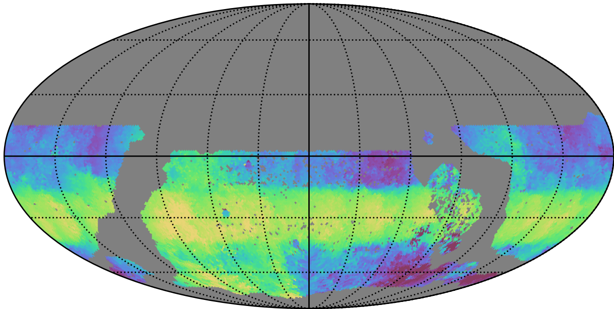
ddf_loaded_half_fl15_v3.4_10yrs WFD u band: Median HA
