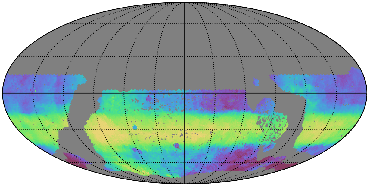
ddf_loaded_half_fl15_v3.4_10yrs WFD r band: Median HA
