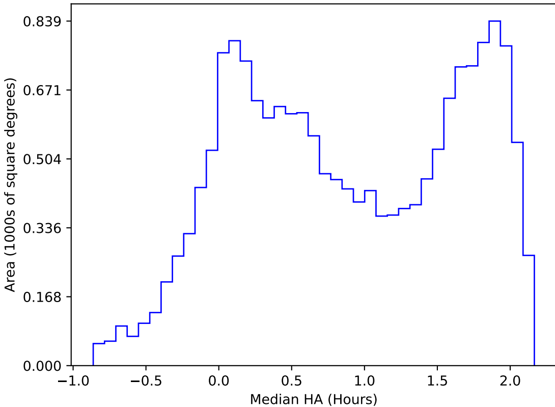
ddf_loaded_half_fl15_v3.4_10yrs WFD r band: Median HA
