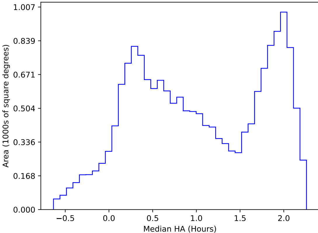
ddf_loaded_half_fl15_v3.4_10yrs WFD i band: Median HA
