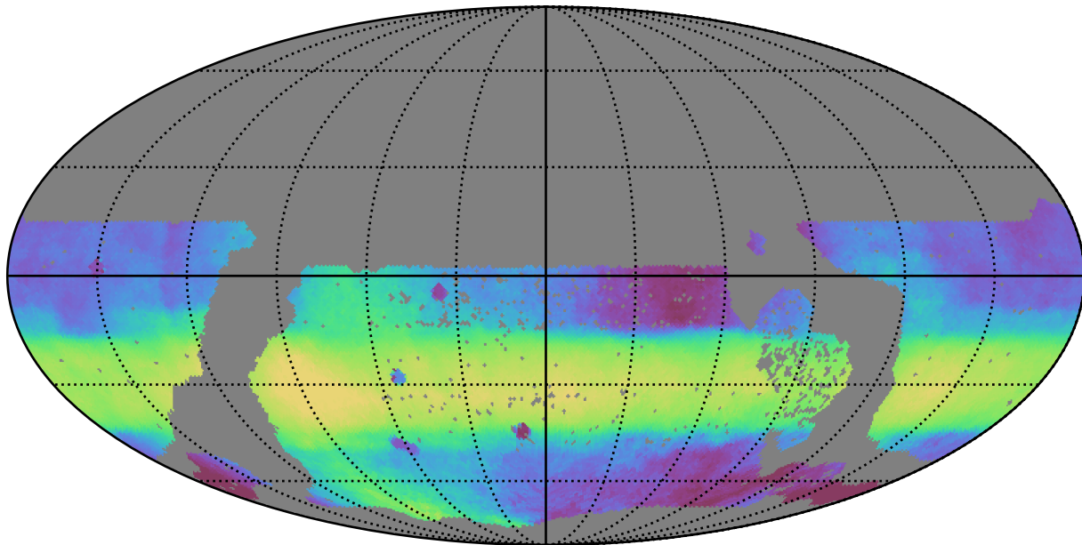
ddf_loaded_half_fl15_v3.4_10yrs WFD all bands: Median HA
