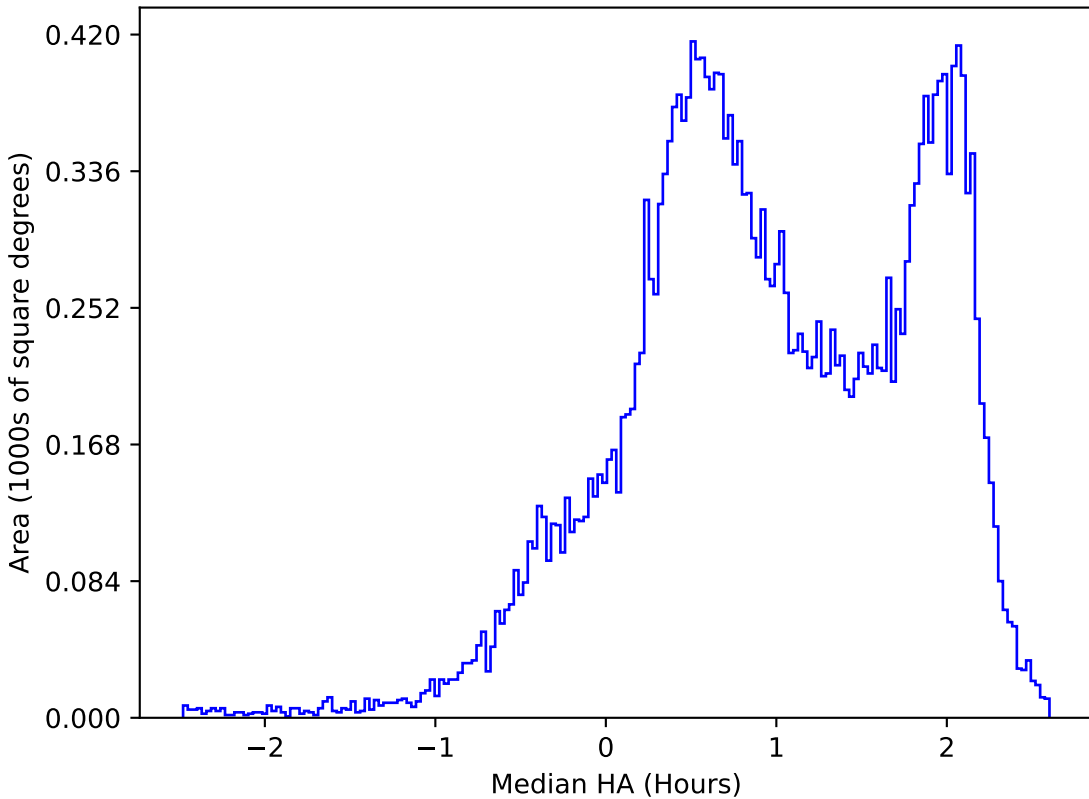
ddf_loaded_half_fl15_v3.4_10yrs All sky z band: Median HA
