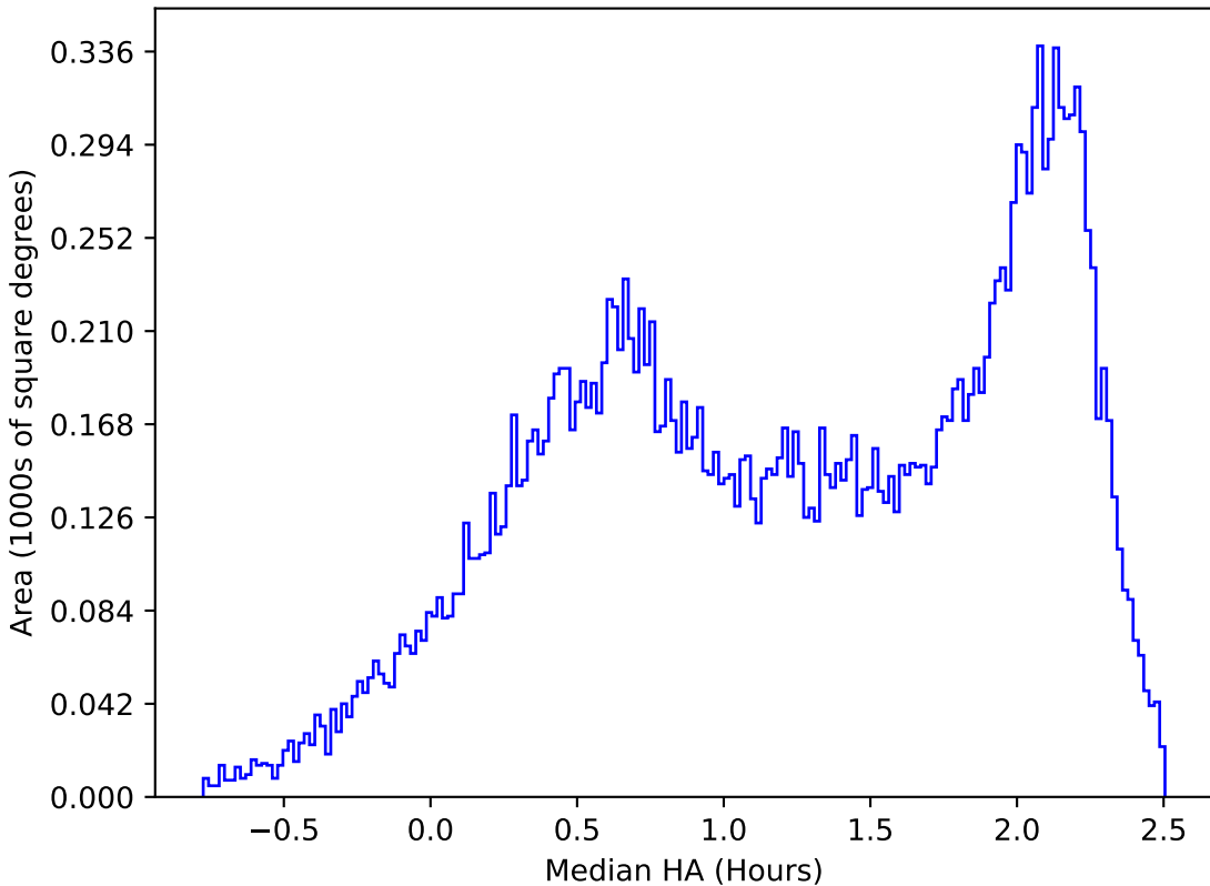
ddf_loaded_half_fl15_v3.4_10yrs All sky y band: Median HA
