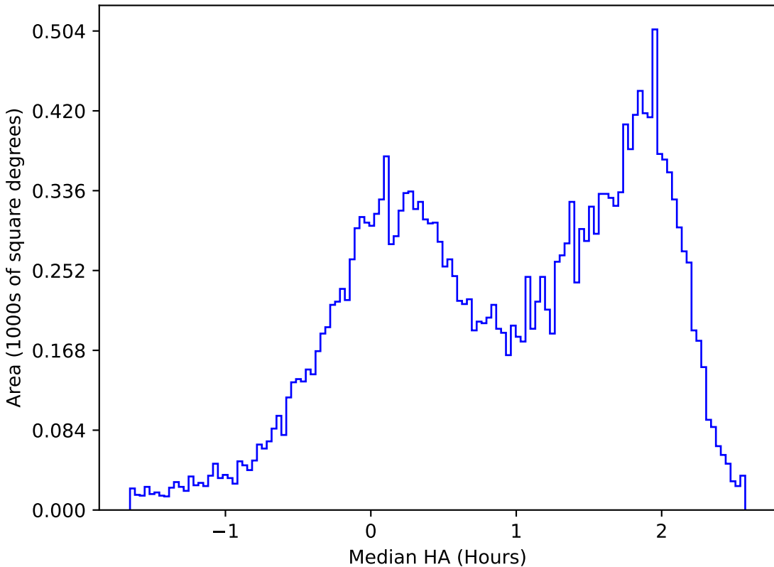
ddf_loaded_half_fl15_v3.4_10yrs All sky u band: Median HA
