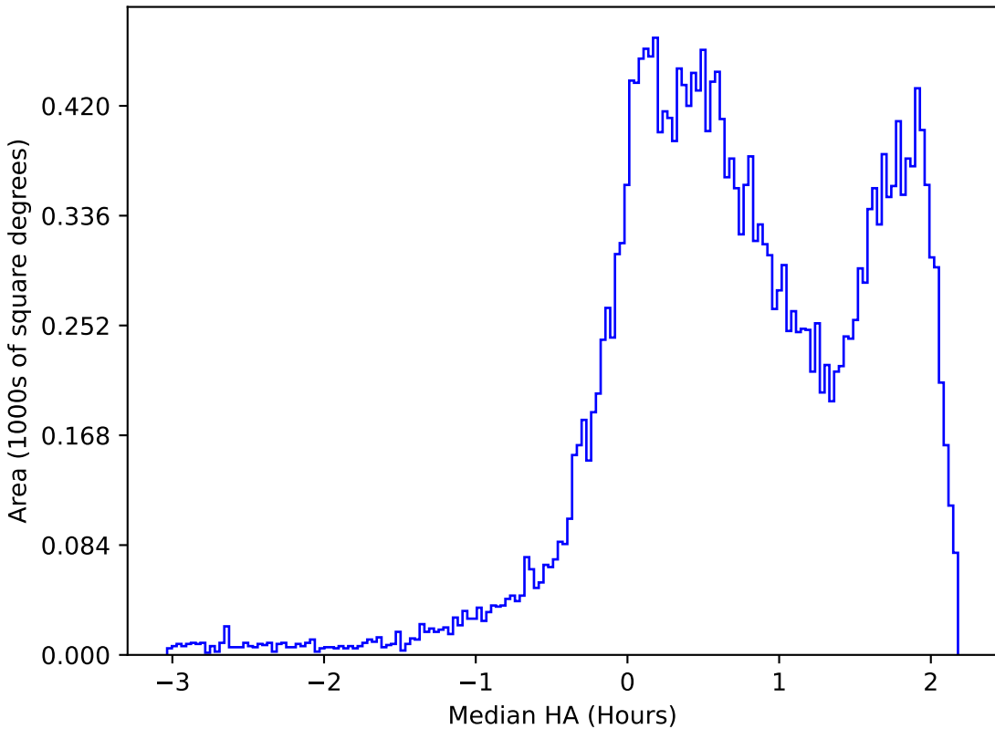
ddf_loaded_half_fl15_v3.4_10yrs All sky r band: Median HA
