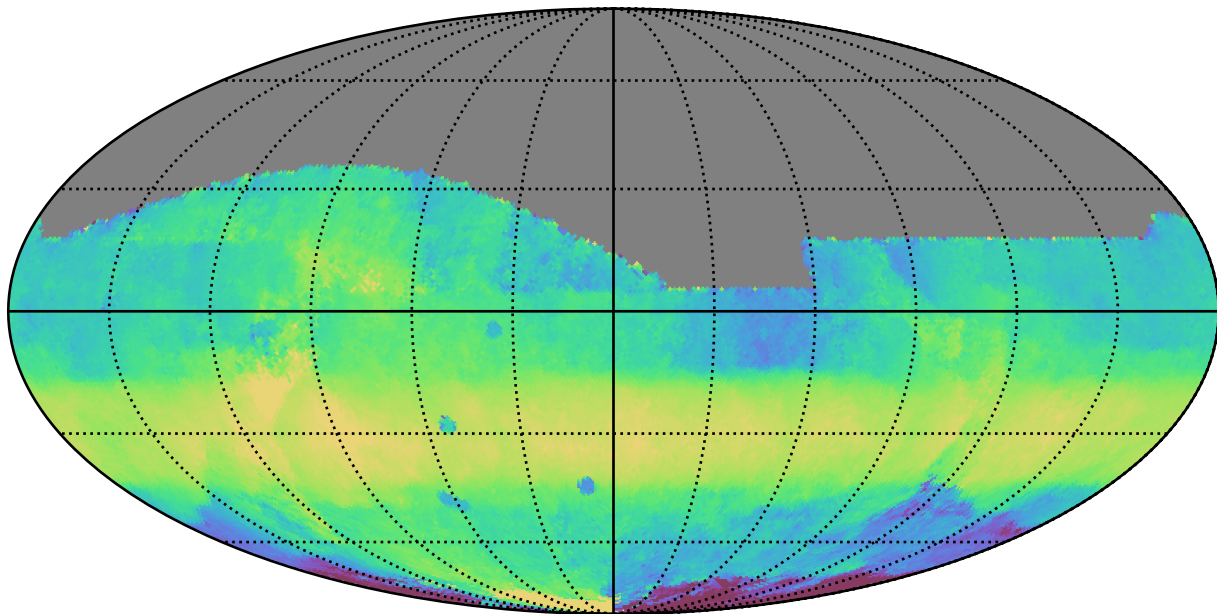
ddf_loaded_half_fl15_v3.4_10yrs All sky i band: Median HA
