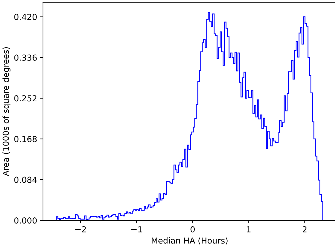
ddf_loaded_half_fl15_v3.4_10yrs All sky i band: Median HA
