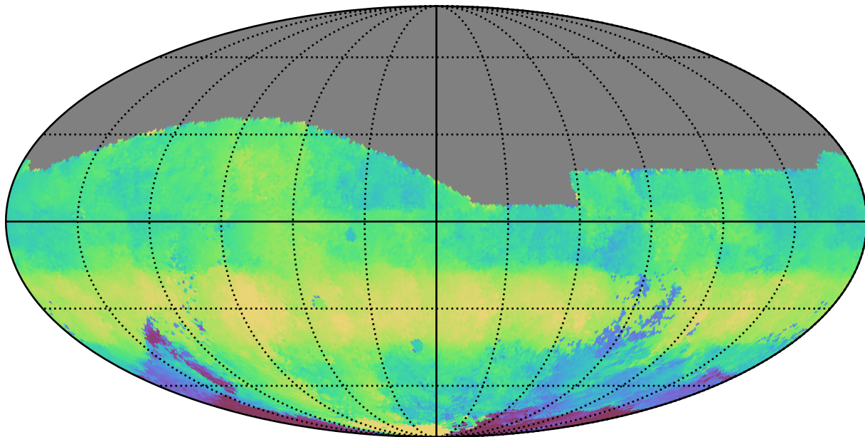
ddf_loaded_half_fl15_v3.4_10yrs All sky g band: Median HA
