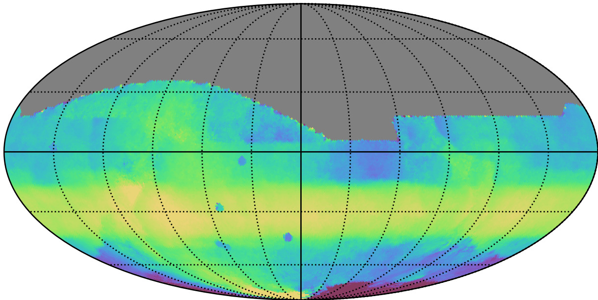
ddf_loaded_half_fl15_v3.4_10yrs All sky all bands: Median HA
