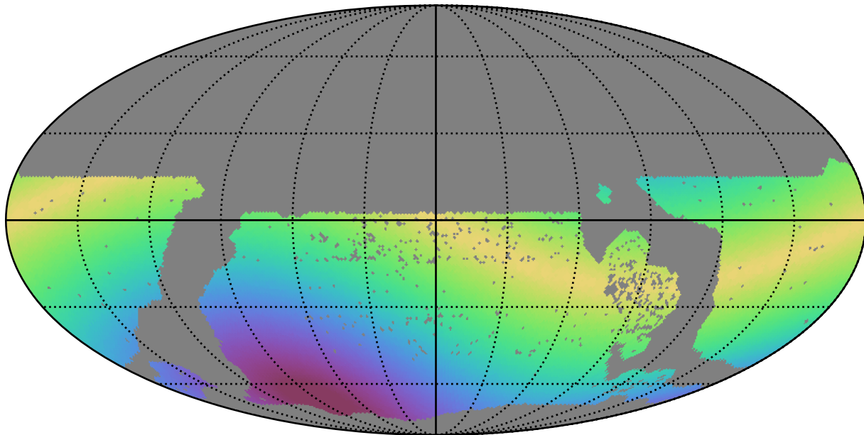
ddf_loaded_half_fl15_v3.4_10yrs WFD z band: Max solarElong
