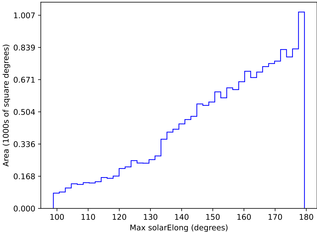
ddf_loaded_half_fl15_v3.4_10yrs WFD z band: Max solarElong
