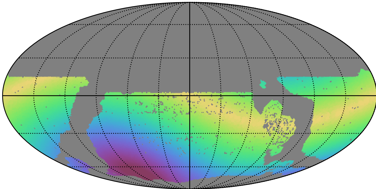
ddf_loaded_half_fl15_v3.4_10yrs WFD y band: Max solarElong
