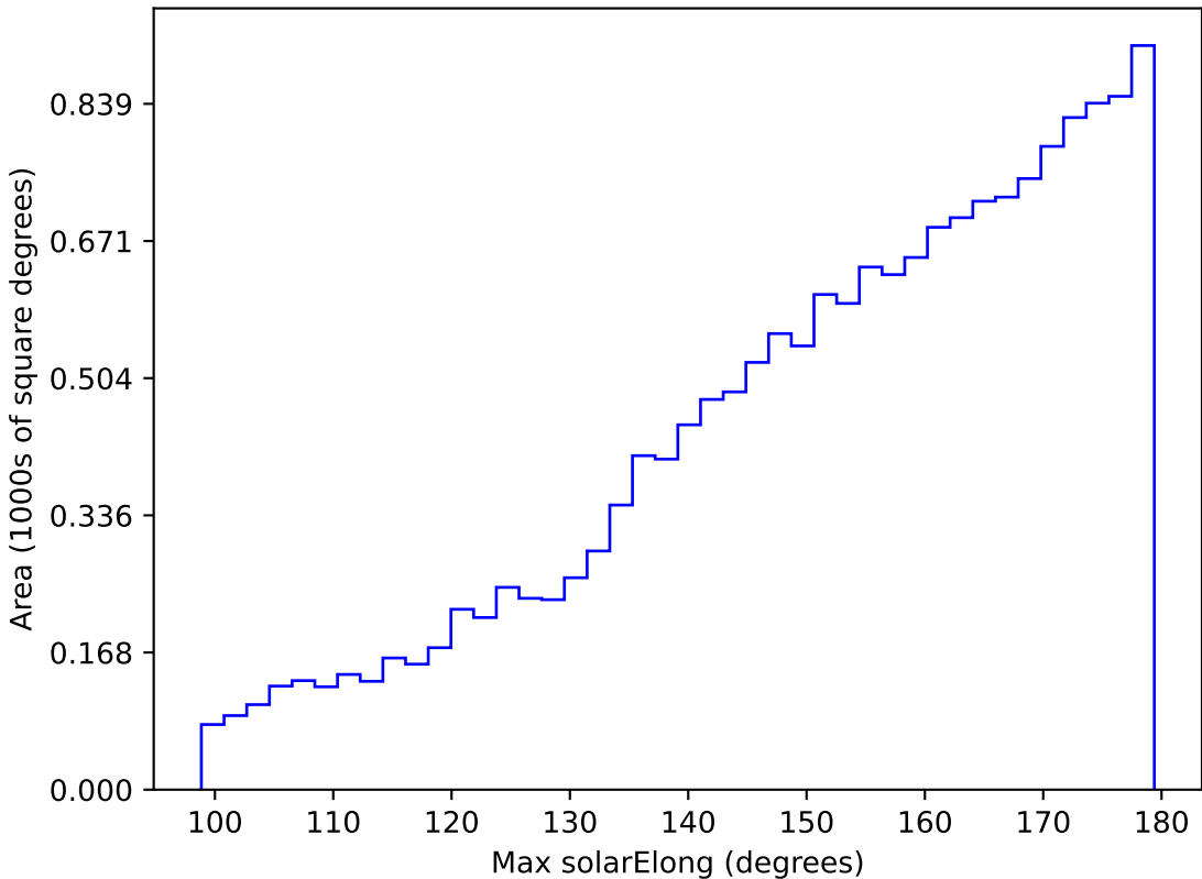
ddf_loaded_half_fl15_v3.4_10yrs WFD y band: Max solarElong
