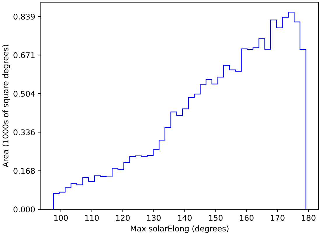
ddf_loaded_half_fl15_v3.4_10yrs WFD u band: Max solarElong
