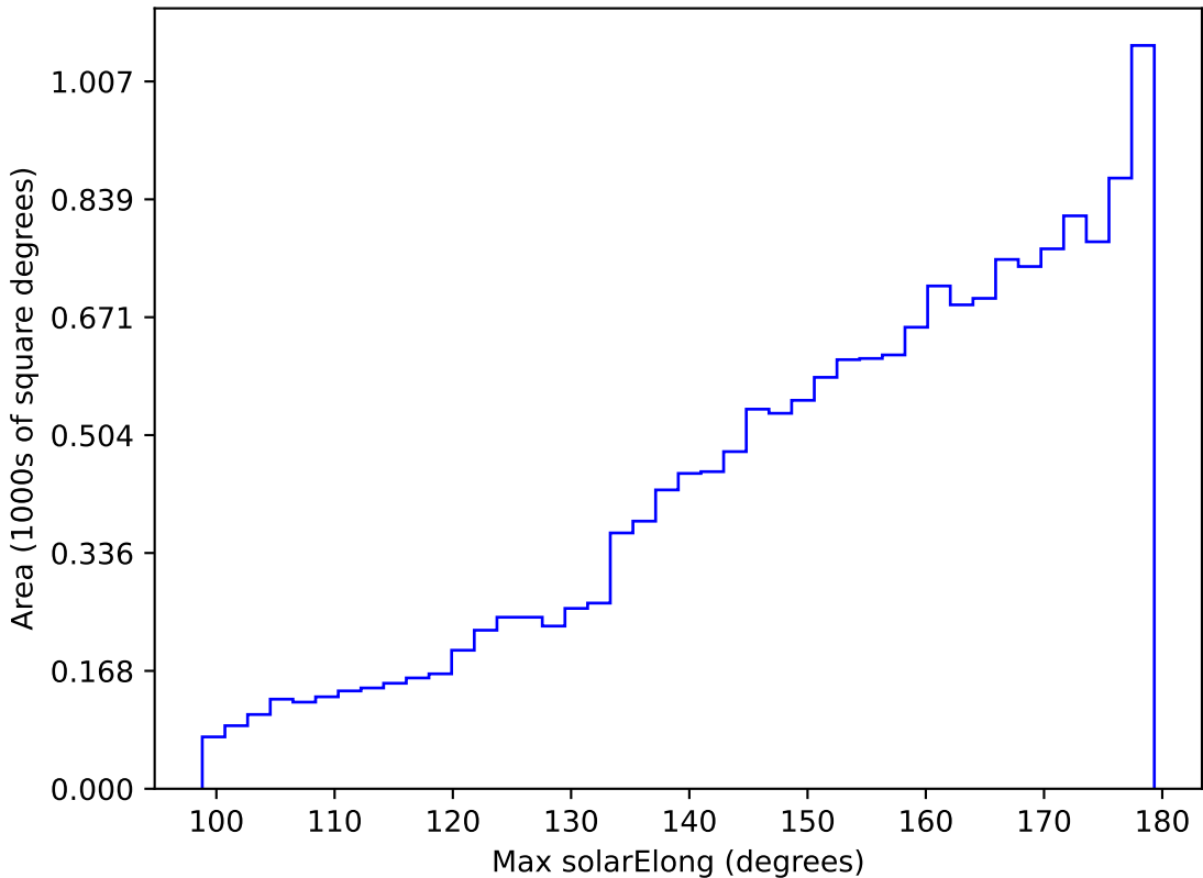
ddf_loaded_half_fl15_v3.4_10yrs WFD i band: Max solarElong
