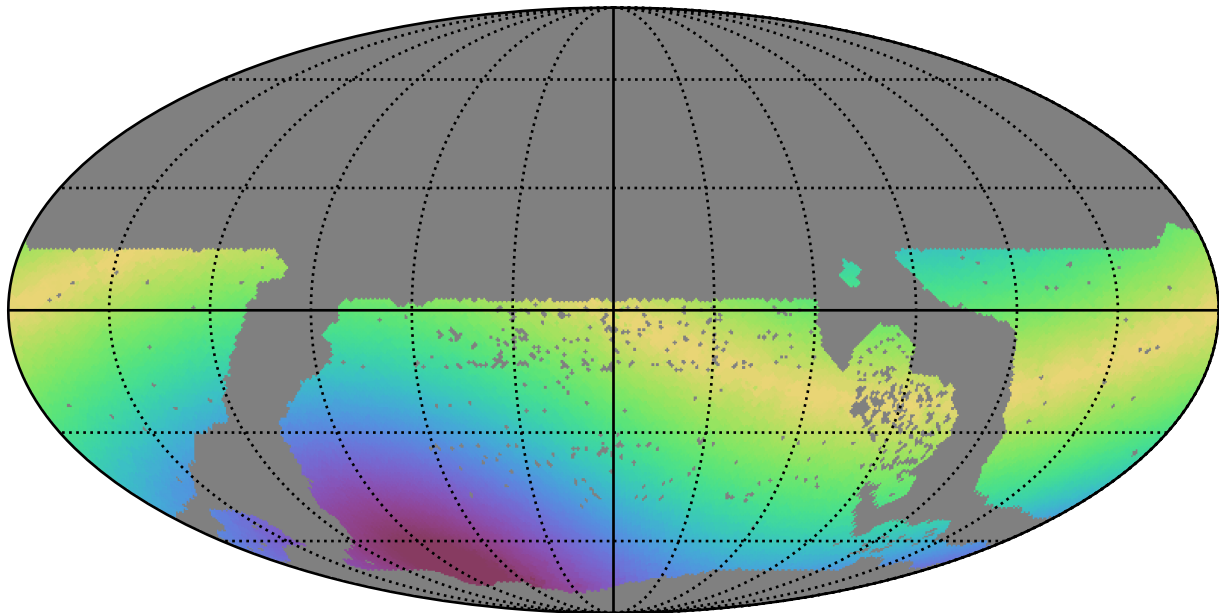
ddf_loaded_half_fl15_v3.4_10yrs WFD g band: Max solarElong
