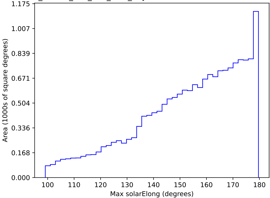
ddf_loaded_half_fl15_v3.4_10yrs WFD all bands: Max solarElong
