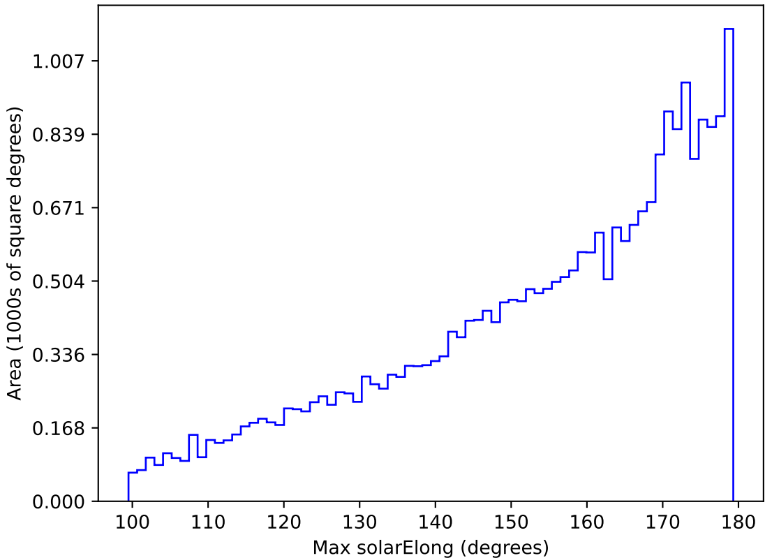
ddf_loaded_half_fl15_v3.4_10yrs All sky z band: Max solarElong
