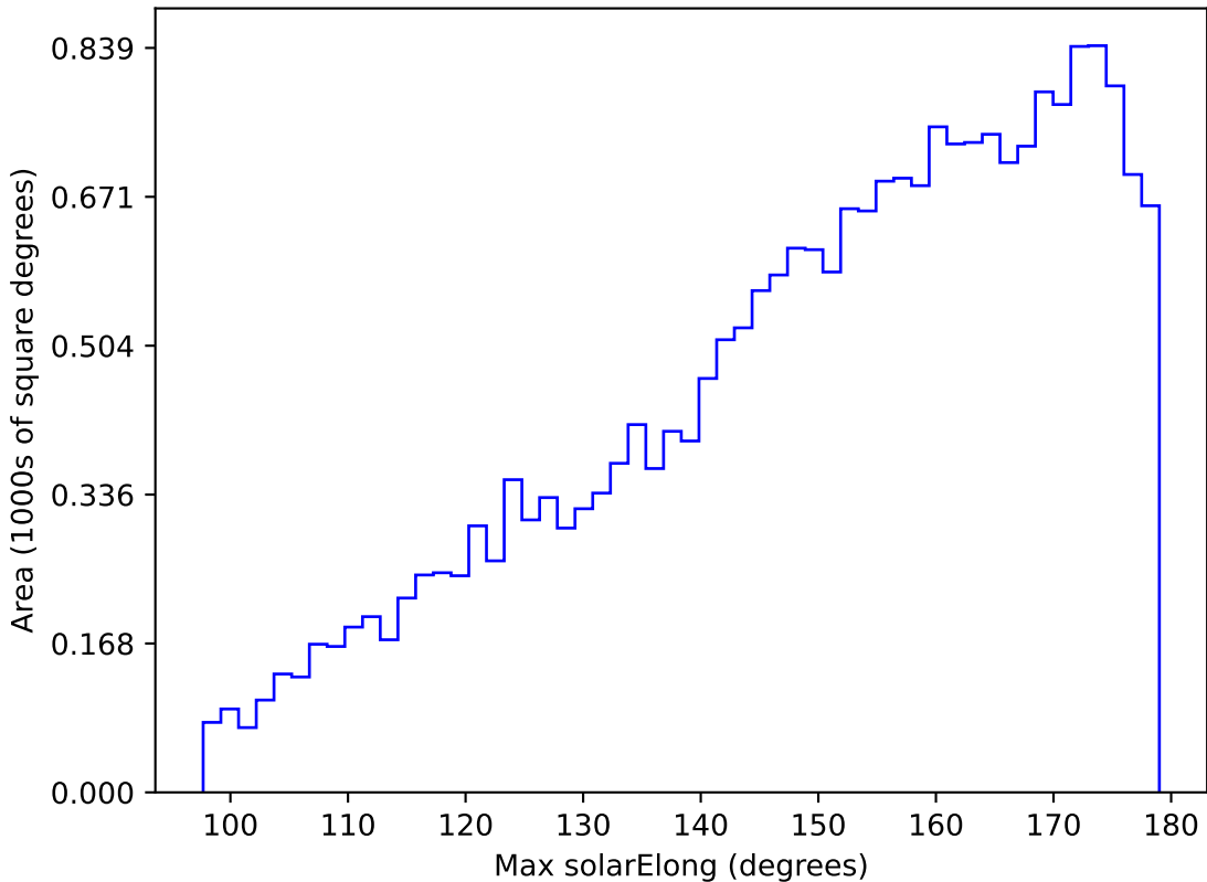
ddf_loaded_half_fl15_v3.4_10yrs All sky u band: Max solarElong
