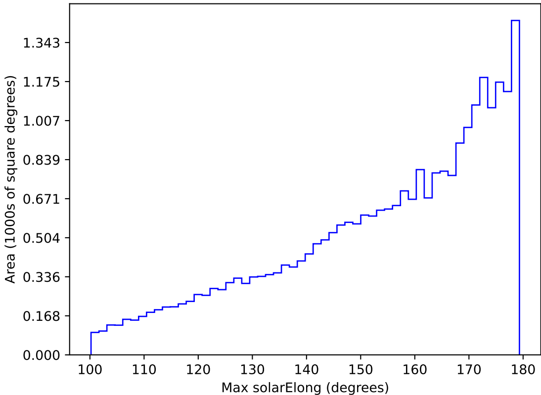
ddf_loaded_half_fl15_v3.4_10yrs All sky r band: Max solarElong
