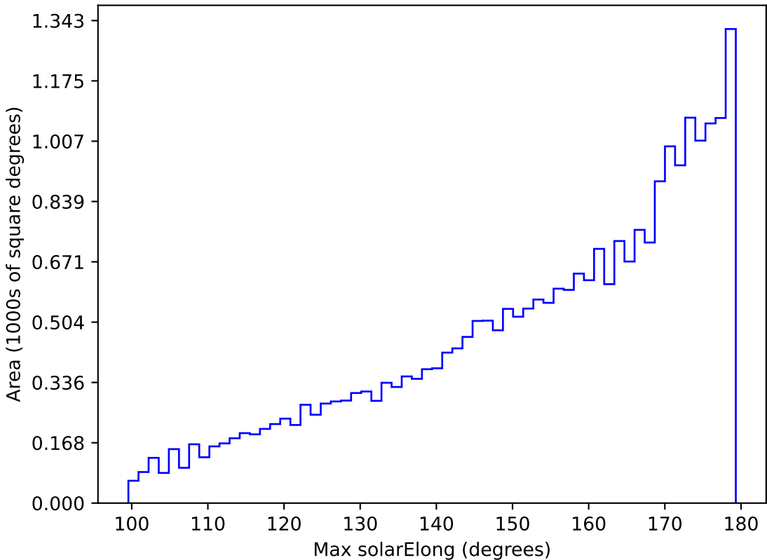
ddf_loaded_half_fl15_v3.4_10yrs All sky i band: Max solarElong
