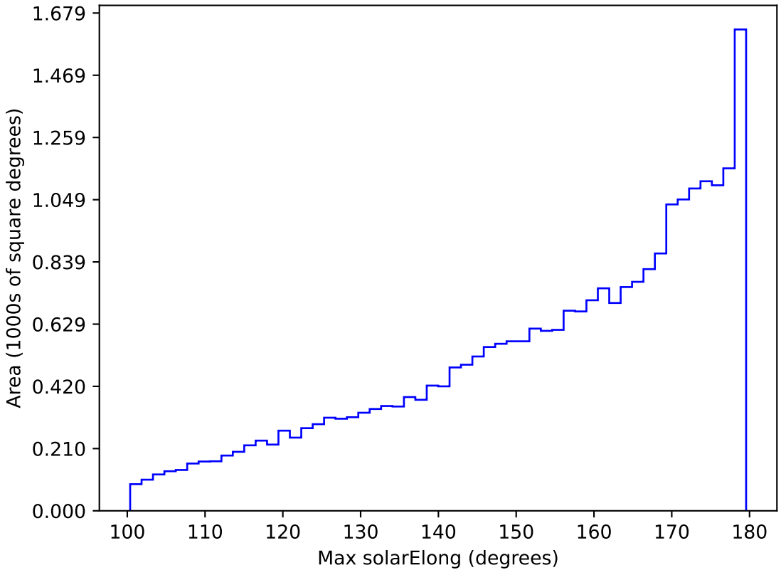
ddf_loaded_half_fl15_v3.4_10yrs All sky all bands: Max solarElong
