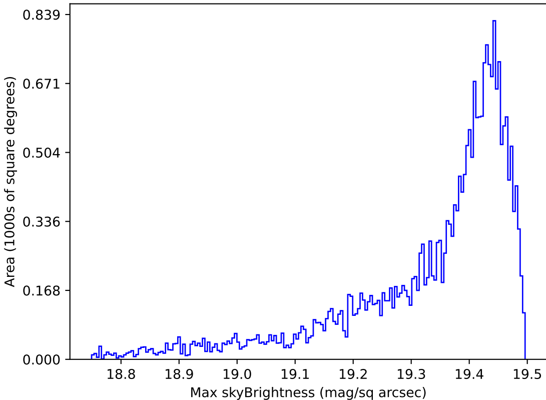
ddf_loaded_half_fl15_v3.4_10yrs Yr 1 z band: Max skyBrightness
