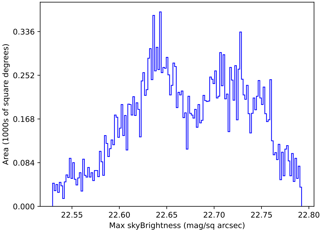
ddf_loaded_half_fl15_v3.4_10yrs Yr 1 u band: Max skyBrightness
