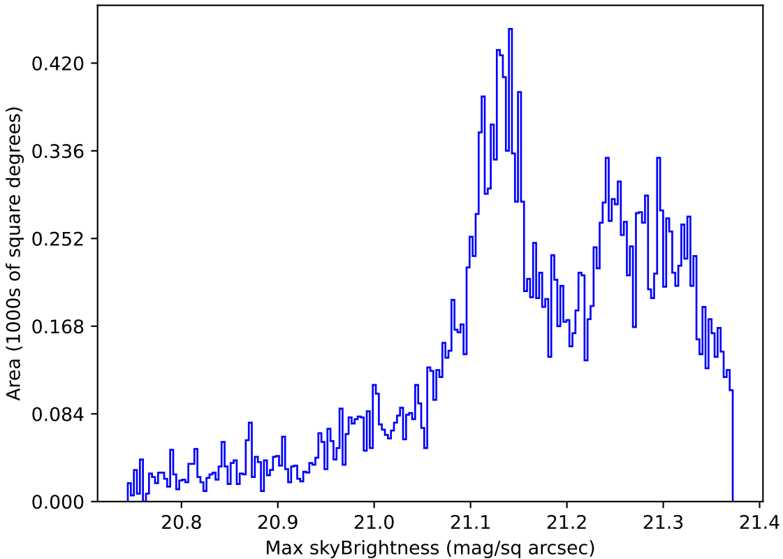
ddf_loaded_half_fl15_v3.4_10yrs Yr 1 r band: Max skyBrightness
