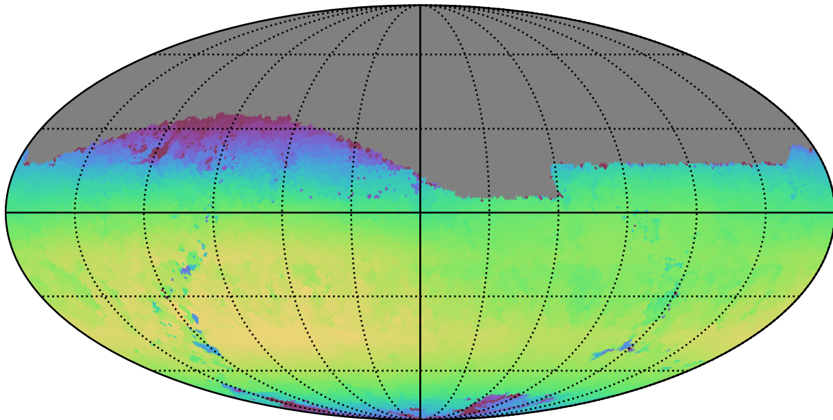
ddf_loaded_half_fl15_v3.4_10yrs Yr 1 i band: Max skyBrightness
