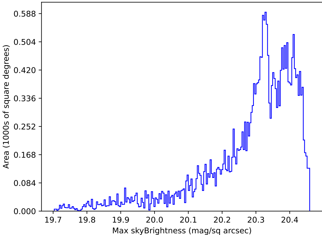
ddf_loaded_half_fl15_v3.4_10yrs Yr 1 i band: Max skyBrightness
