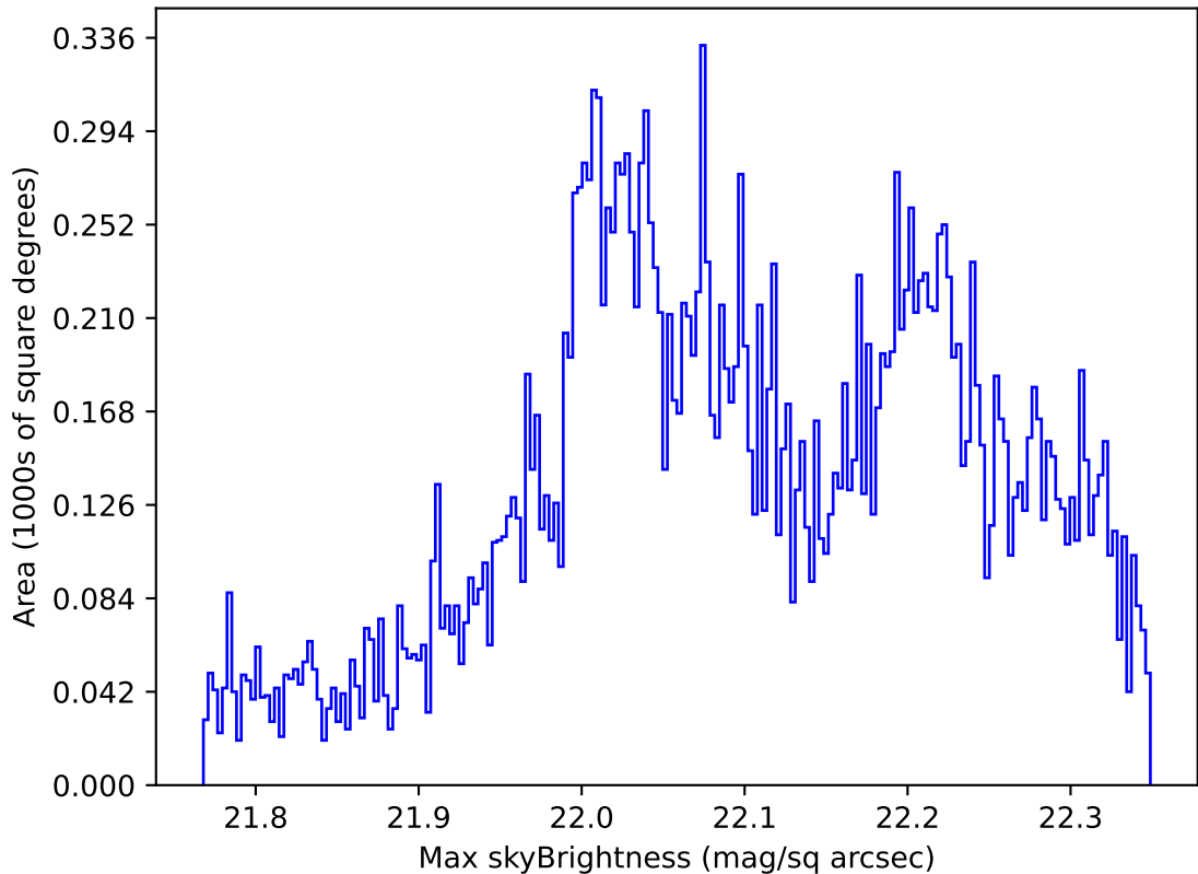
ddf_loaded_half_fl15_v3.4_10yrs Yr 1 g band: Max skyBrightness
