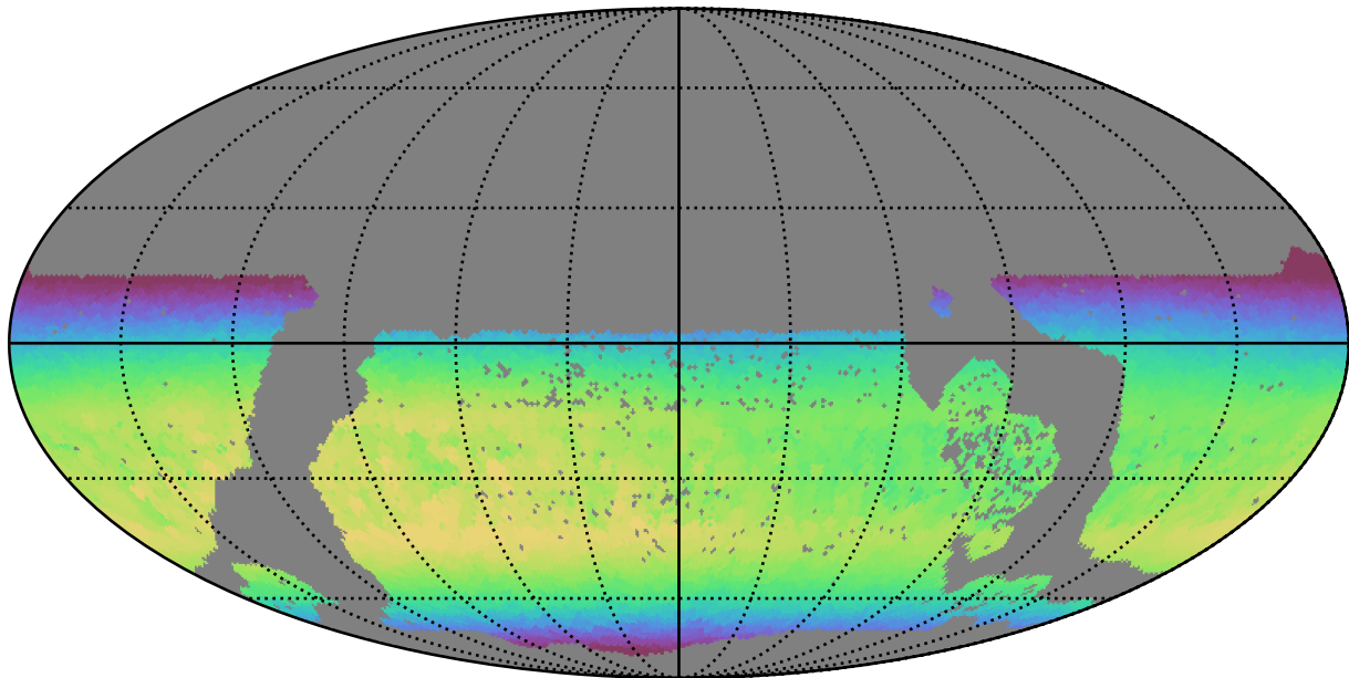
ddf_loaded_half_fl15_v3.4_10yrs WFD z band: Max skyBrightness
