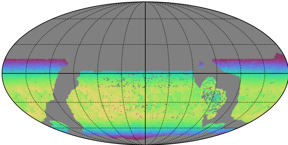
ddf_loaded_half_fl15_v3.4_10yrs WFD y band: Max skyBrightness
