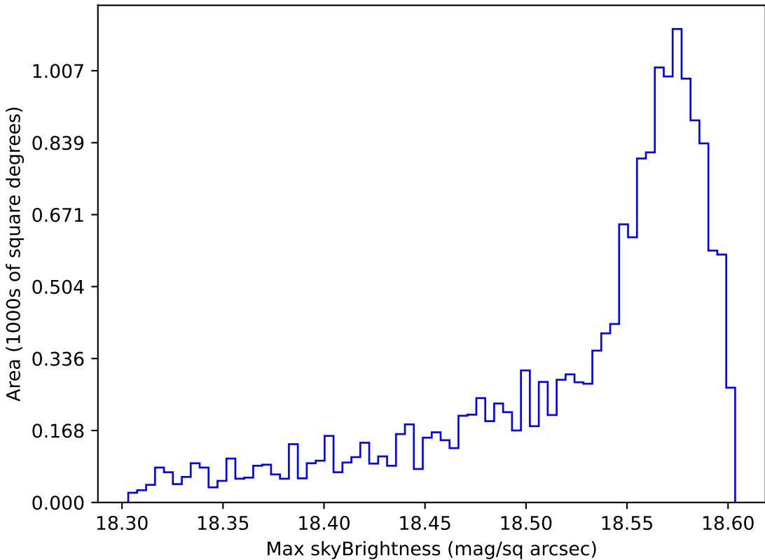
ddf_loaded_half_fl15_v3.4_10yrs WFD y band: Max skyBrightness
