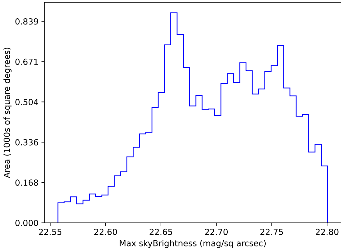
ddf_loaded_half_fl15_v3.4_10yrs WFD u band: Max skyBrightness
