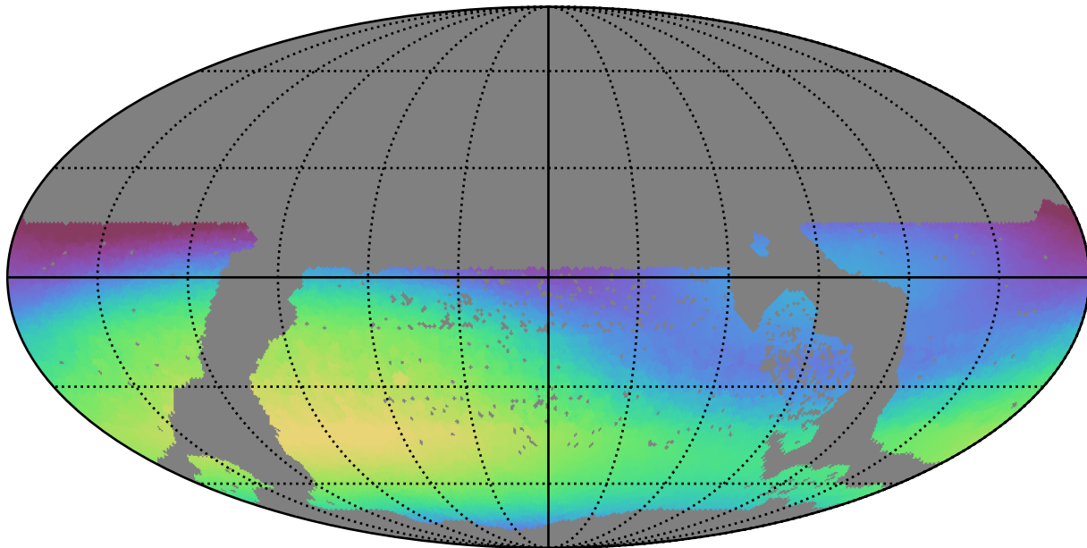
ddf_loaded_half_fl15_v3.4_10yrs WFD r band: Max skyBrightness
