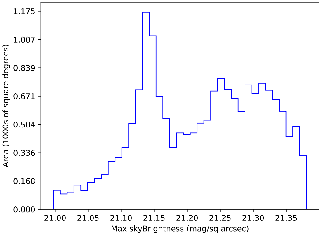
ddf_loaded_half_fl15_v3.4_10yrs WFD r band: Max skyBrightness
