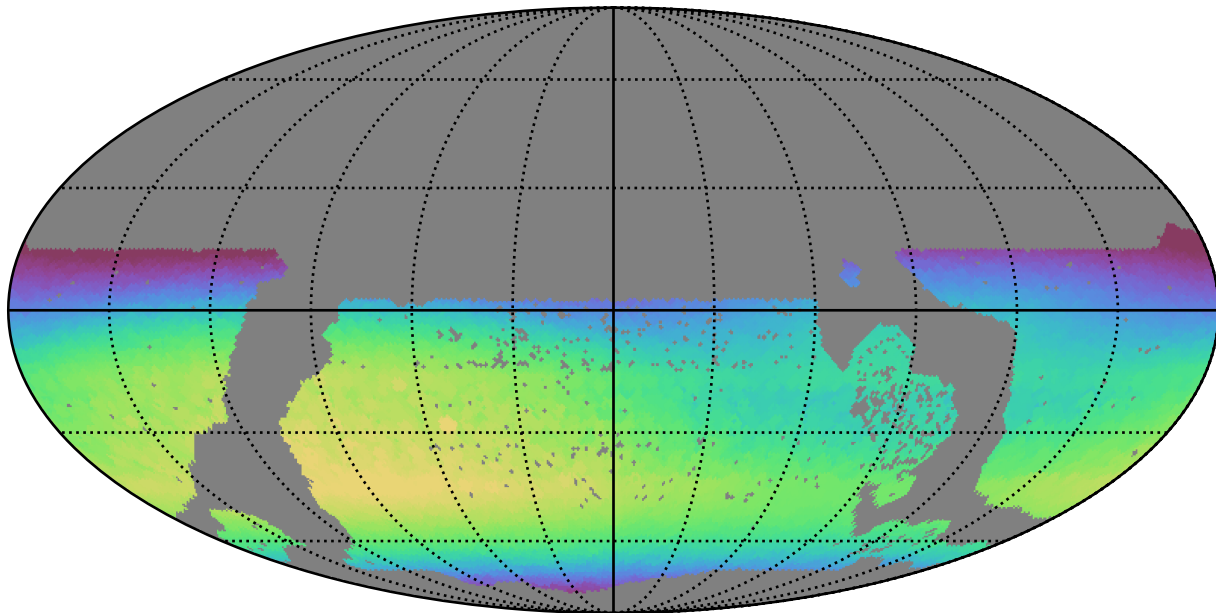
ddf_loaded_half_fl15_v3.4_10yrs WFD i band: Max skyBrightness
